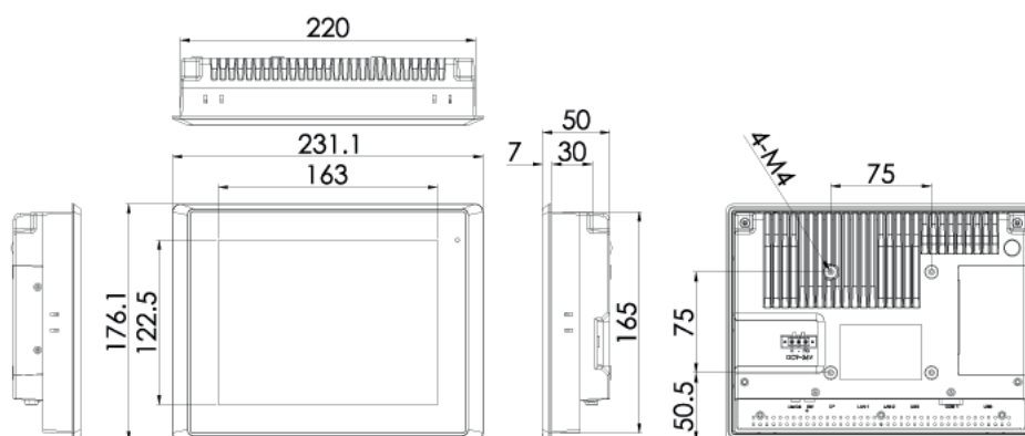
MMI5088B - 8.1"
