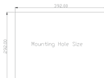
MMI5168B -15.6''
