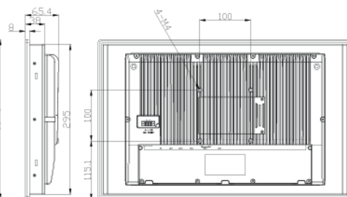
MMI5188B -18.5''
