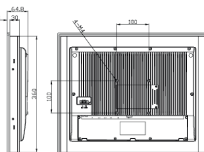
MMI5198B -19''
