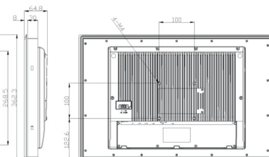
MMI5218B -21.5''
