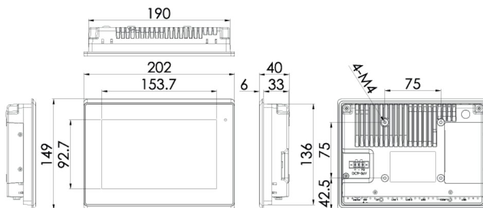
MMI5078B - 7"
